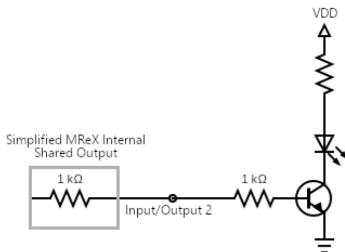
DMReX Output 2 Shared with Input 2
