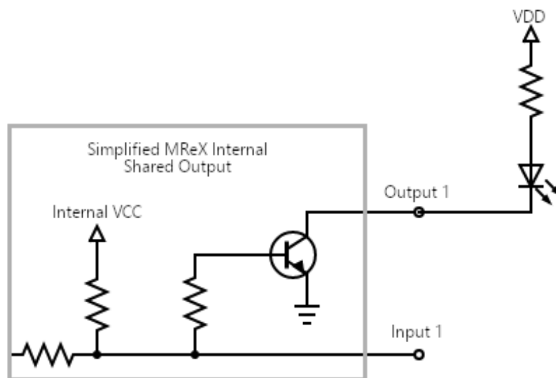
DMReX Output 1 Shared with Input 1
